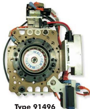
Type 91496 Multiflansch multi flange
